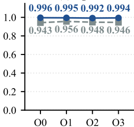
(b) Nginx
