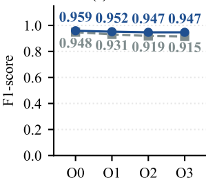
(c) Coreutils
