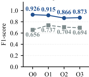
(a) OpenSSL
